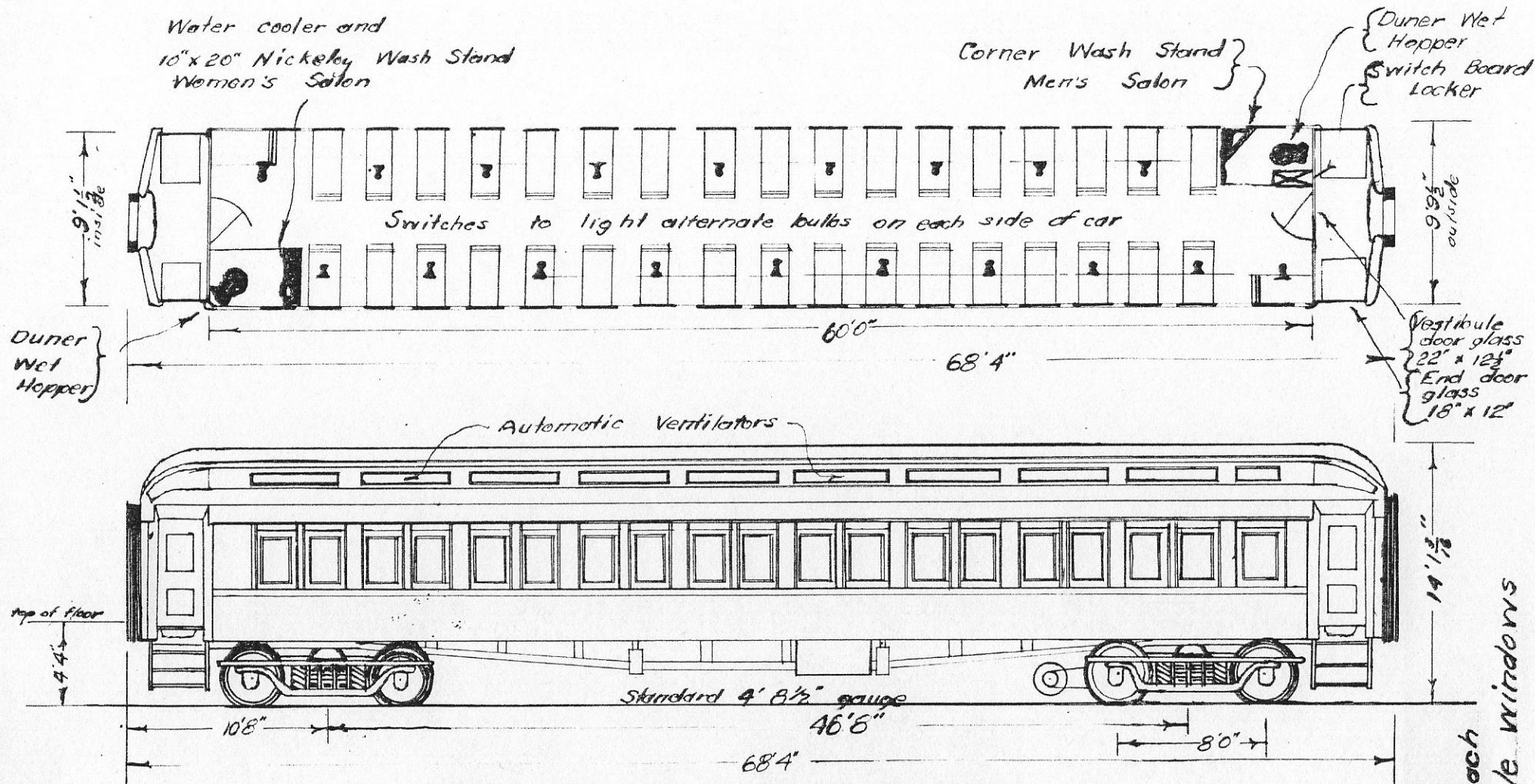
A.R.R. - Passenger Coaches - #20 and 21
