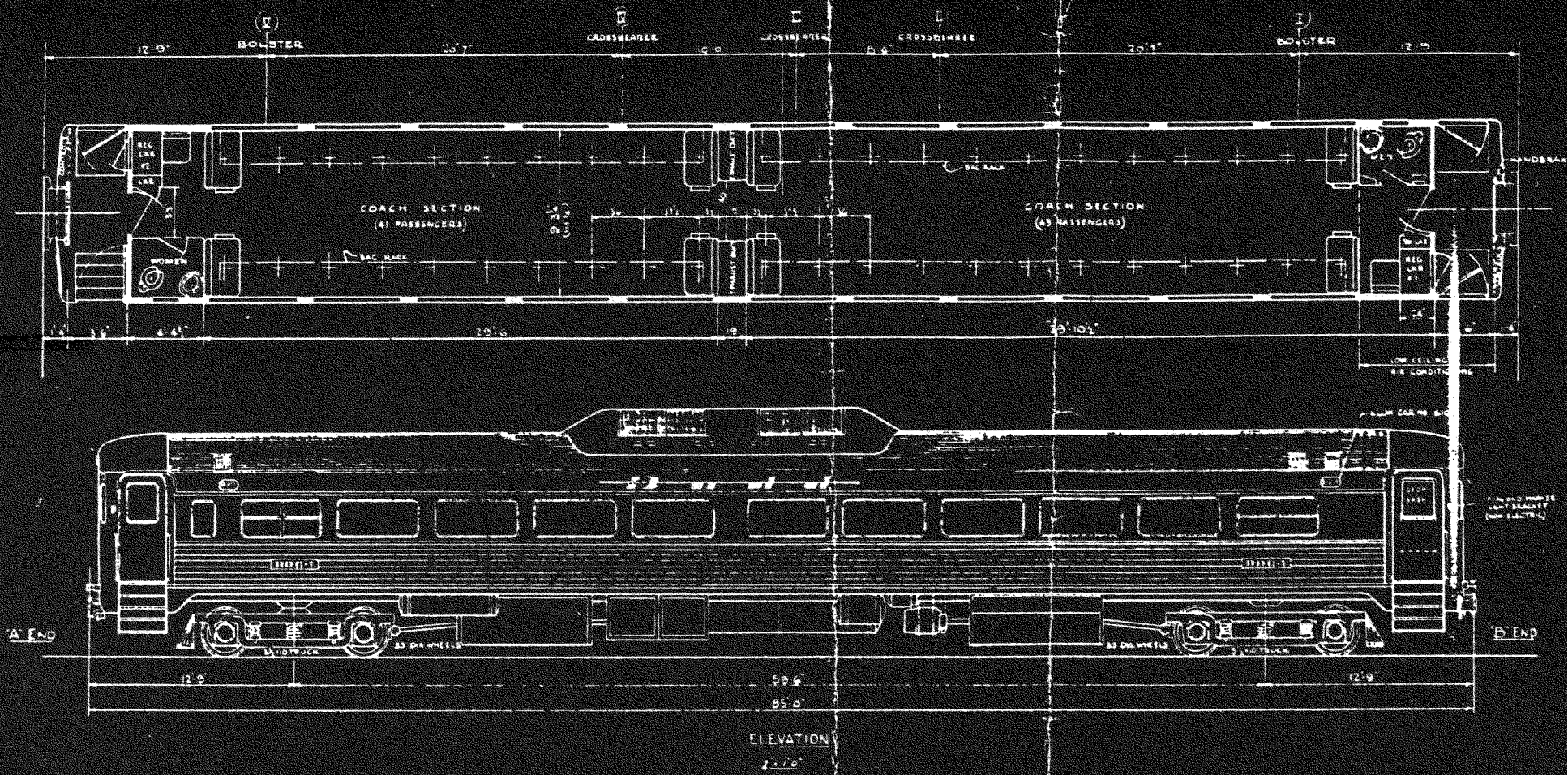
Plan and elevation, RDC-1
