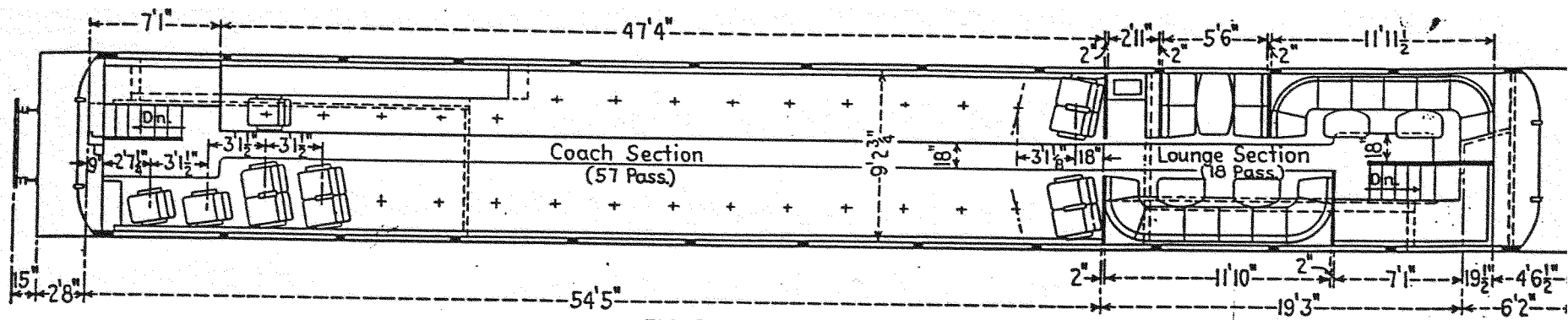
FLOOR PLAN-UPPER LEVEL
