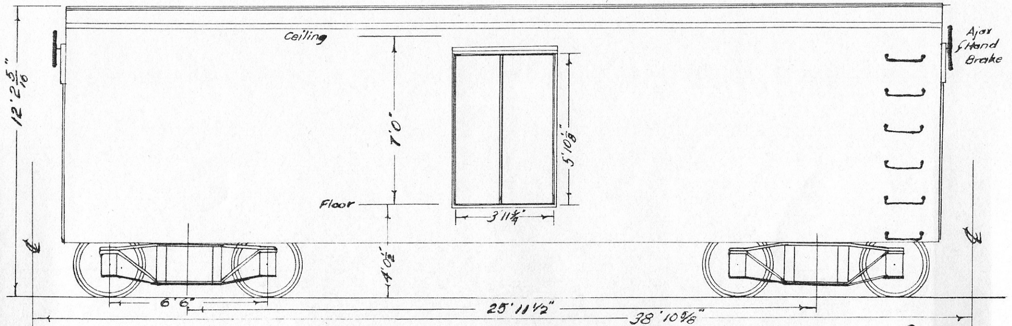
Freight Equipment - Hot Cars (Green) - # 71-79 (inc.)
